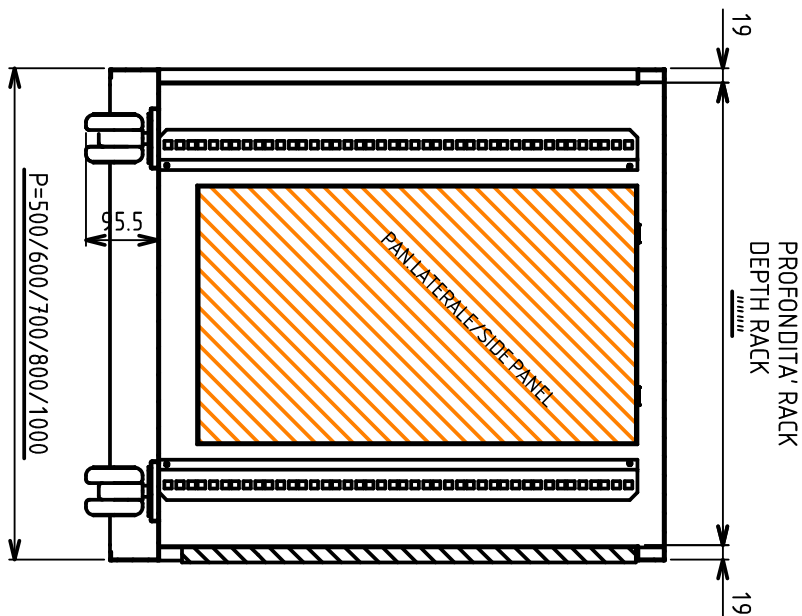
VISTA LATERALE/SIDE VIEW
