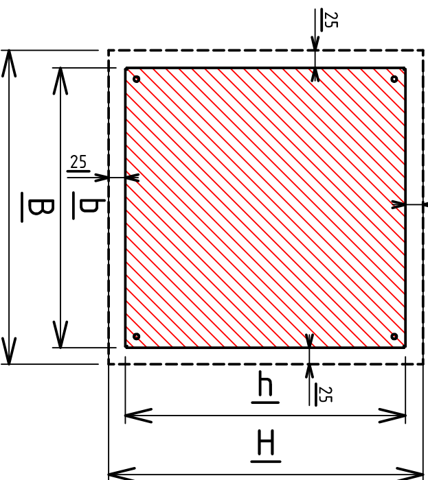
VISTA LATERALE/SIDE VIEW
